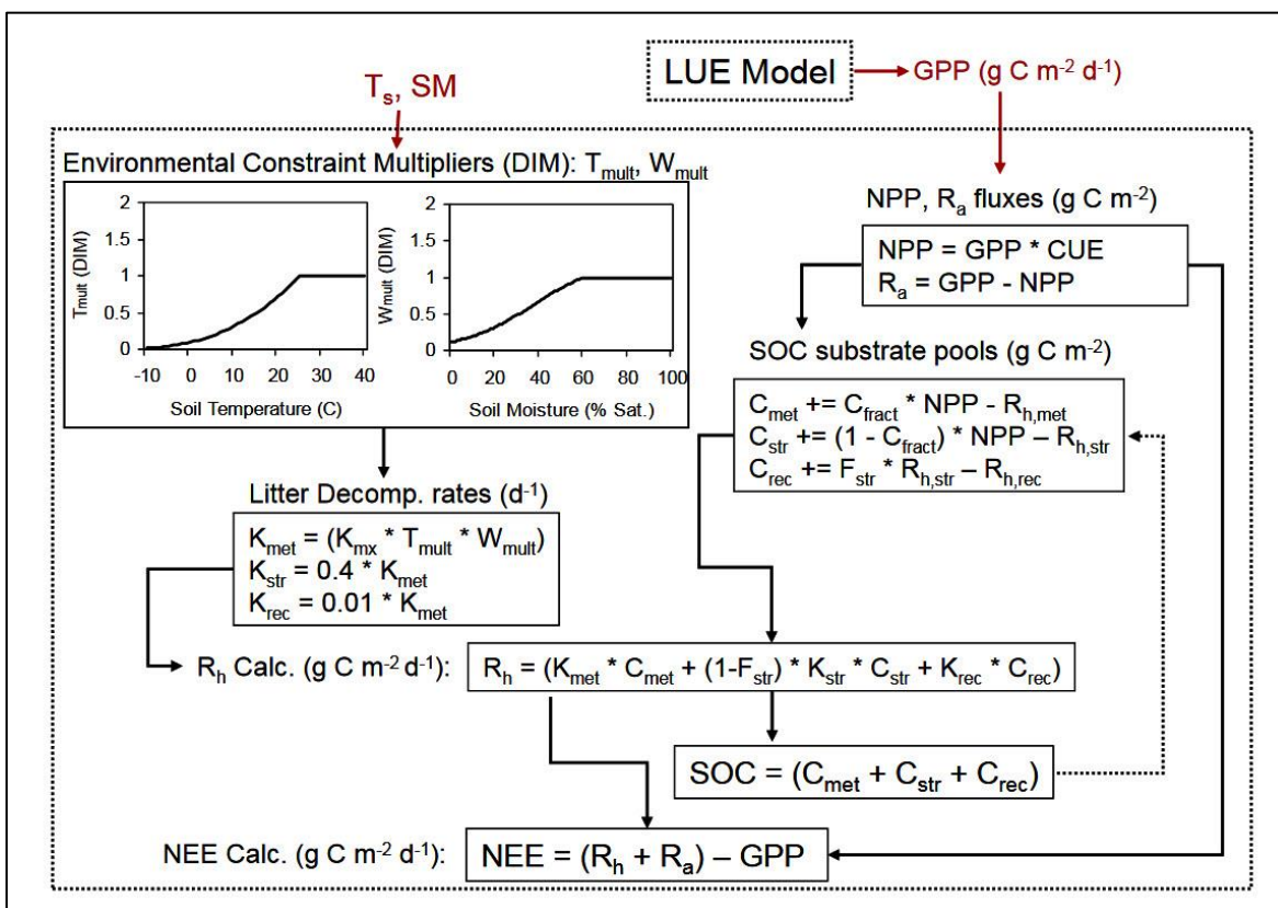
Figure 3. Terrestrial Carbon Flux Model for Estimating NEE
