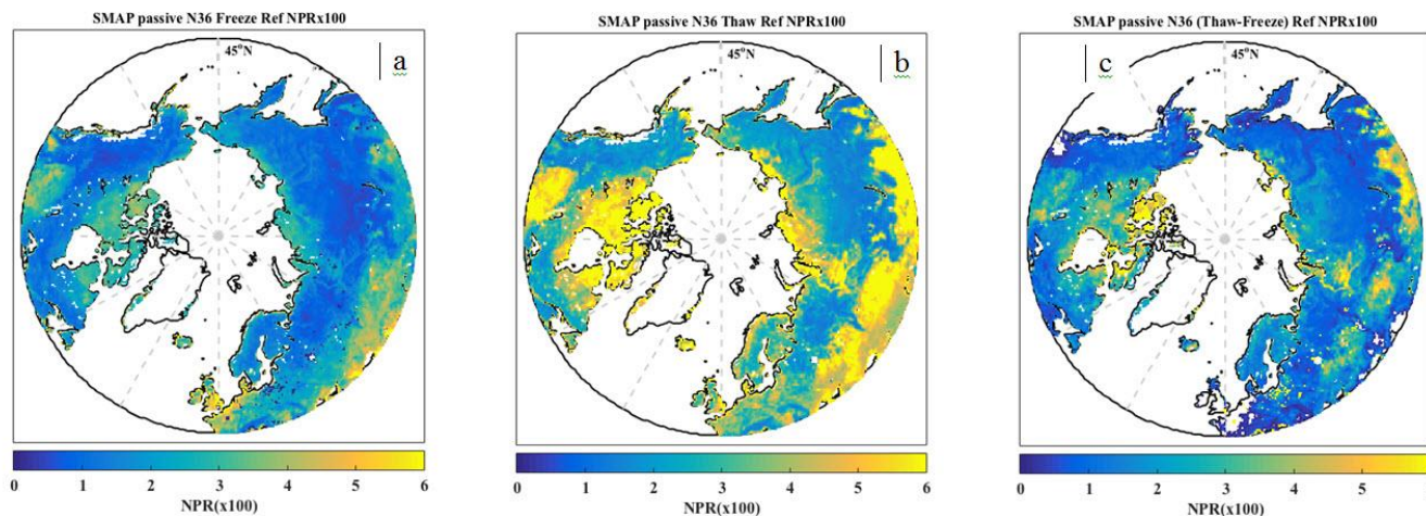
Figure 4. Initial SMAP Freeze and Thaw NPR References. SMAP radiometer (a) freeze and (b) thaw references; (c) reference difference between panels (a) and (b). Units are NPR scaled by 100.
