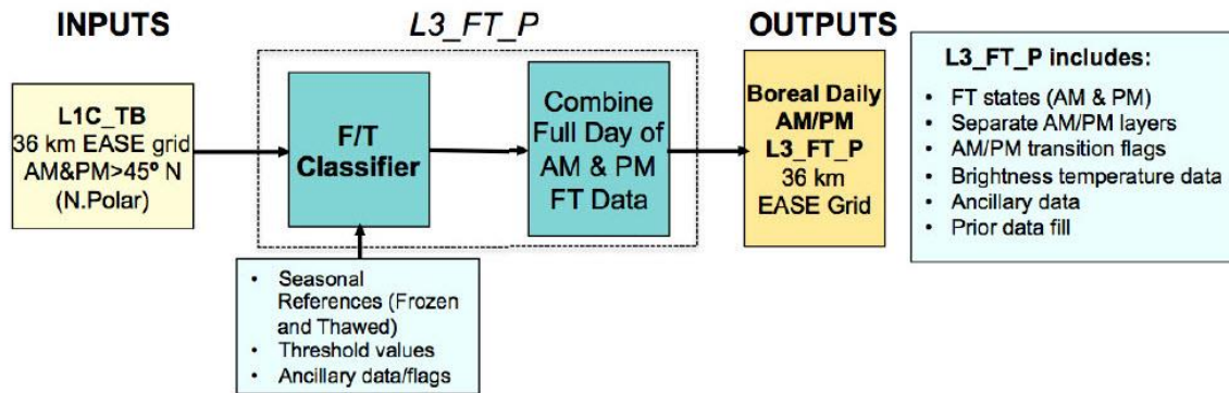
Figure 4. Processing Sequence for the L3 Freeze/Thaw Radiometer Product (SPL3FTP)
