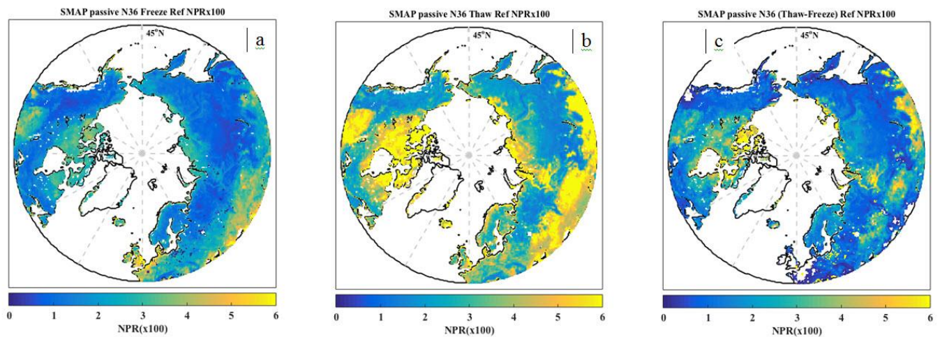
Figure 3. Initial SMAP Freeze and Thaw NPR References. SMAP radiometer (a) freeze and (b) thaw references; (c) reference difference between panels (a) and (b). Units are NPR scaled by 100.
