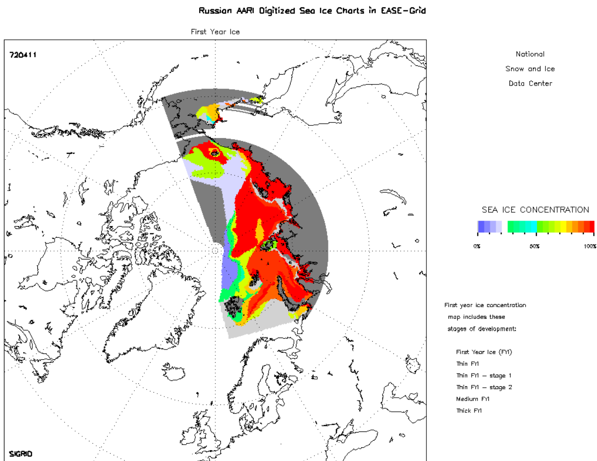
Figure 5. ASCII SIGRID file regrided and displayed to EASE-Grid, SIGRIDINF :RFAA:099:A7680002400:BO410213:C0015: D06CTCABCCNCD: SIGRID01:E98201049999:F001 =K002:L021163:M0213 :R19CT92CA808799CB208...02LL...
