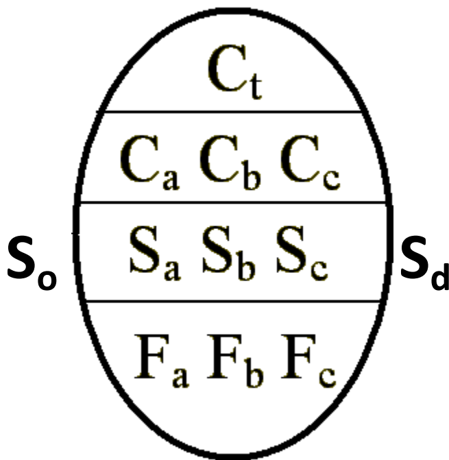
Figure A - 1. WMO Egg Code Ice Symbology
