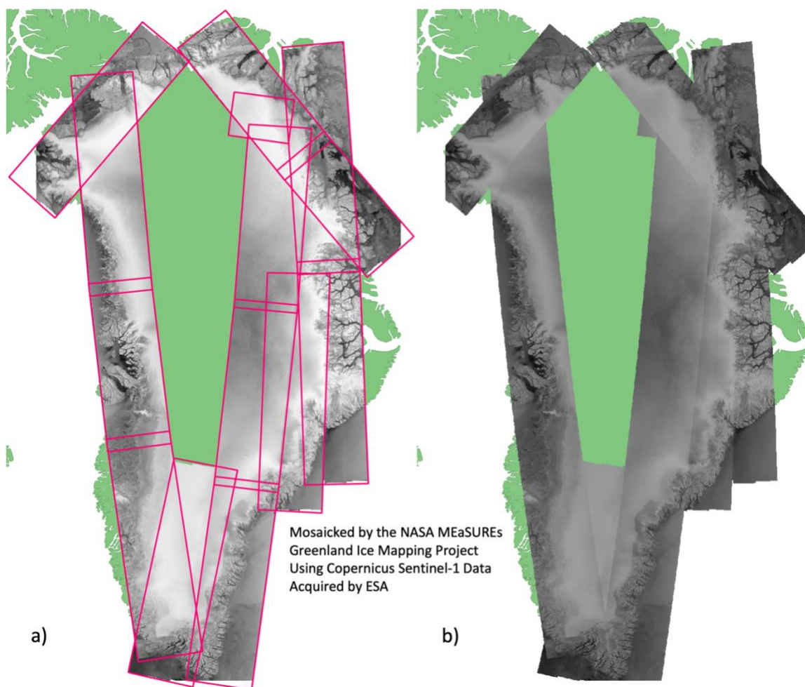
Figure 1. Sample mosaics of data collected from 06 November 2019 to 11 November 2019 (file names beginning with GL_S1bks_mosaic_06Nov19_11Nov19_ ), displayed here over Greenland's continental outline (not included in the data). In a) , the pink polygons are contained in the shapefile and denote the individual images used in the mosaic; attributes for each polygon indicate their date, track, orbit, and particular satellite (S1 A/B). The background image is the sigma0 JPEG Quicklook mosaic for the same dates. In b) , the sigma0 GeoTIFF mosaic for the same dates is displayed. All products contain modified Copernicus Sentinel data, acquired and processed by the European Space Agency, distributed through the Alaska Satellite Facility, and mosaicked by I. Joughin.
