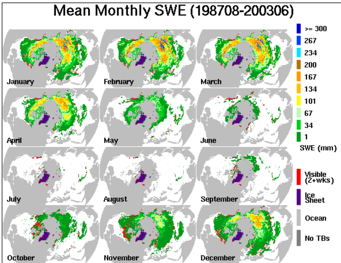
Figure 6. Northern Hemisphere monthly long-term average snow water equivalent (mm) from SSM/I, with additional area indicated as snow by Northern Hemisphere EASE-Grid weekly snow cover in red, (August 1987 - June 2003).
