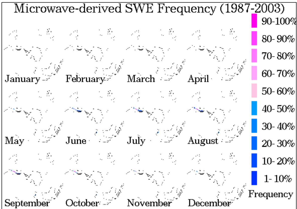
Figure 15. Southern Hemisphere long-term snow cover frequencies (1987-2003) derived from SSM/I-derived SWE frequency of occurrence. Areas with "likely" snow are limited to the Andes Mountains region and New Zealand. Frequency thresholds are a function of month (20% for October through May, 7% for June through September). These frequency maps are used for Southern Hemisphere Processing Steps, Step 5.
