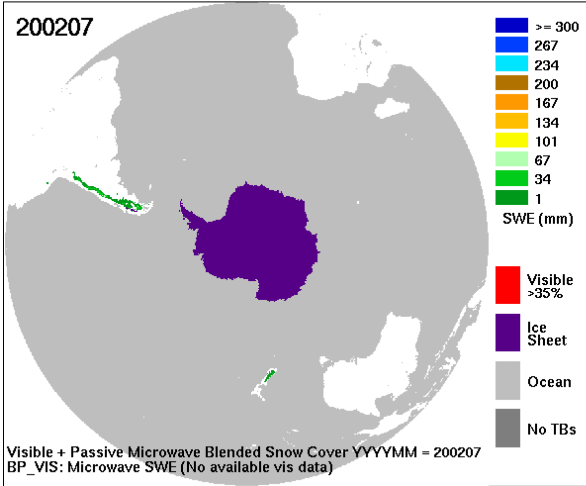
Figure 7. Southern Hemisphere average snow water equivalent (mm) from passive microwave, July, 2002.
