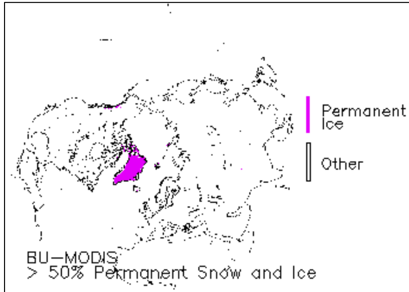
Figure 12. Northern Hemisphere permanent ice mask, derived from BU-MODIS land cover data.
