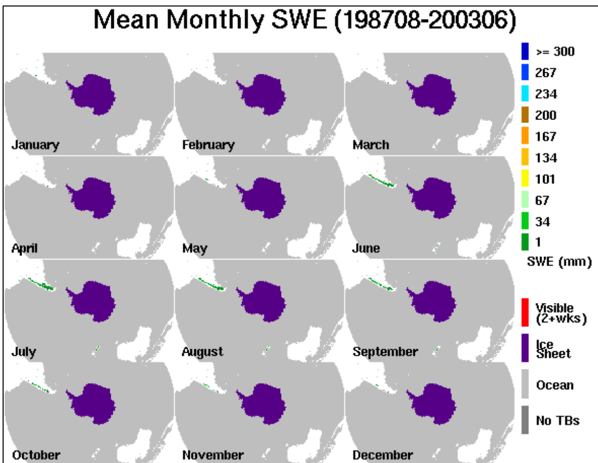
Figure 9. Southern Hemisphere monthly long-term average snow water equivalent (mm) from SSM/I,
