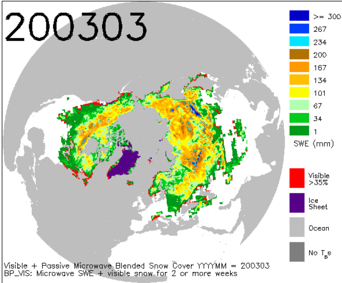
Figure 3. Northern Hemisphere average snow water equivalent (mm) from passive microwave, with additional area indicated as snow by Northern Hemisphere EASE-Grid weekly snow cover in red, March, 2003.
