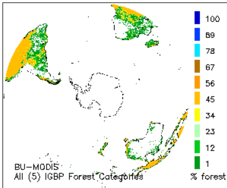
Figure 11. Southern Hemisphere forest percent mask, derived from BU-MODIS Land Cover data
