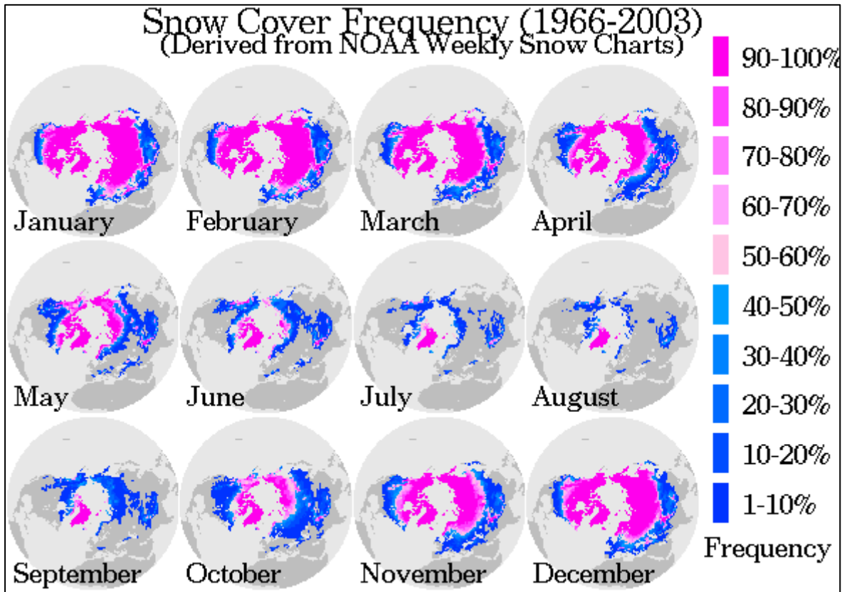
Figure 14. Long-term snow cover frequencies (1966-2003) derived from Northern Hemisphere EASE-Grid Weekly Snow Cover and Sea Ice Extent Version 2 data, used for Processing Steps, Step 5.
