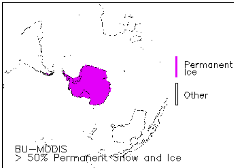
Figure 13. Southern Hemisphere permanent ice mask, derived from BU-MODIS land cover data.
