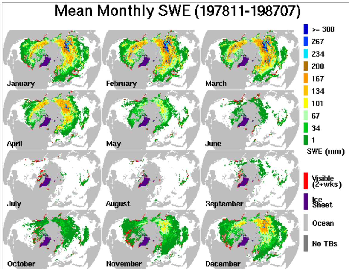
Figure 5. Northern Hemisphere monthly long-term average snow water equivalent (mm) from SMMR, with additional area indicated as snow by Northern Hemisphere EASE-Grid weekly snow cover in red, (November 1978 - July 1987).
