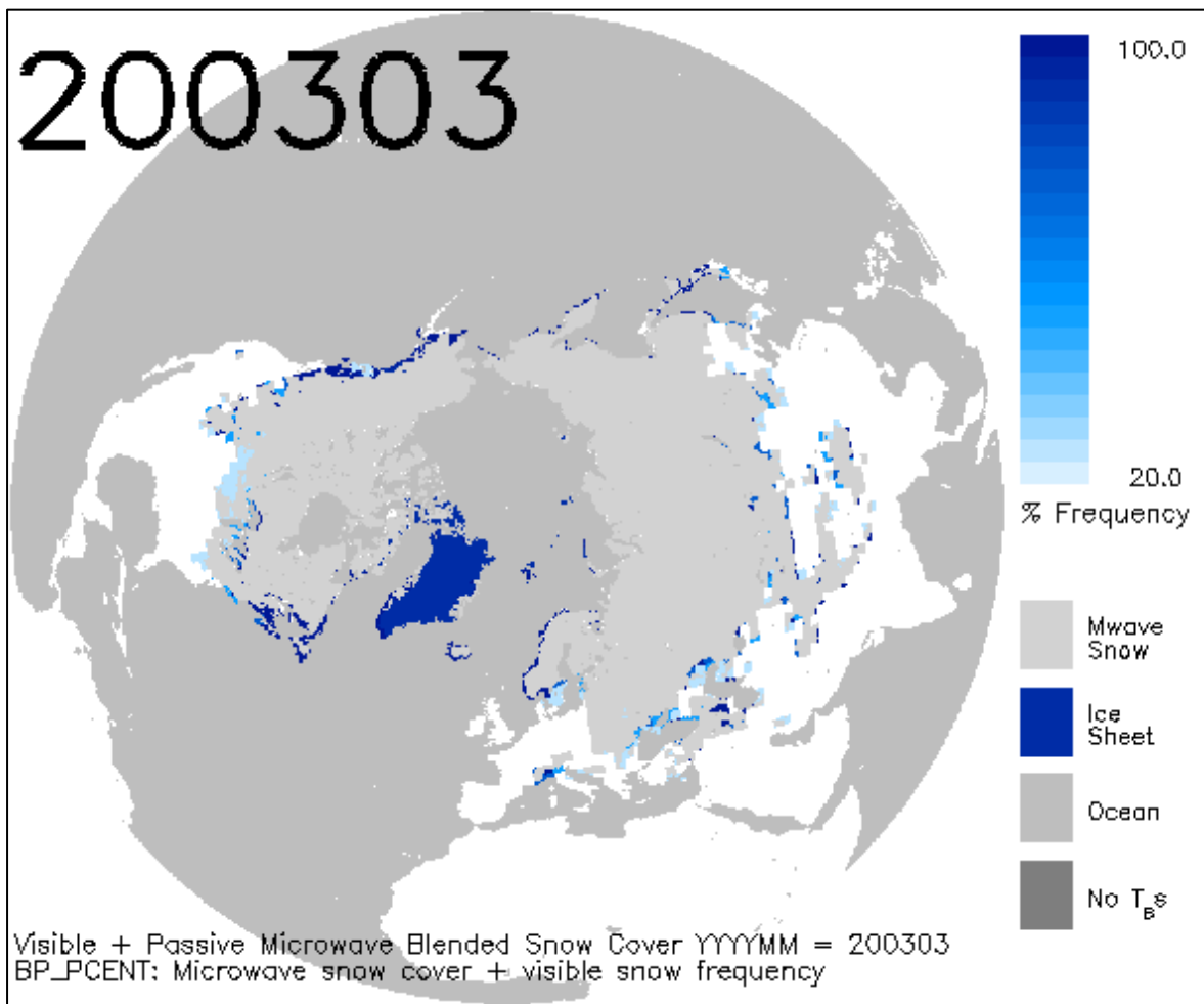
Figure 4. Northern Hemisphere snow extent from passive microwave (gray), with snow-cover frequency for the month from Northern Hemisphere EASE-Grid weekly snow cover (blue shades), March, 2003.
