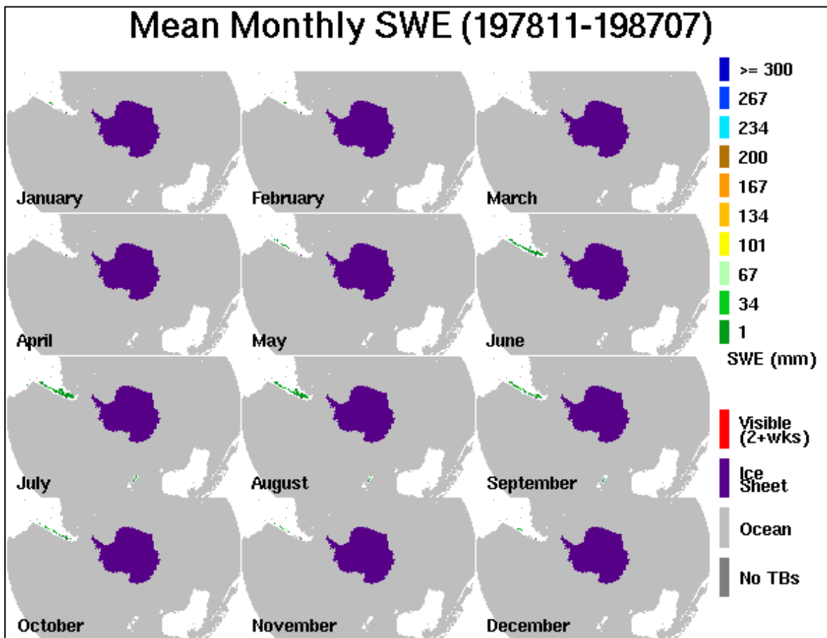
Figure 8. Southern Hemisphere monthly long-term average snow water equivalent (mm) from SMMR, (November 1978 - July 1987).
