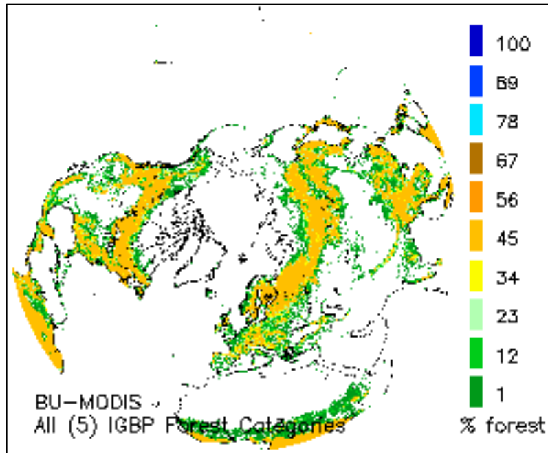
Figure 10. Northern Hemisphere forest percent mask, derived from BU-MODIS Land Cover data
