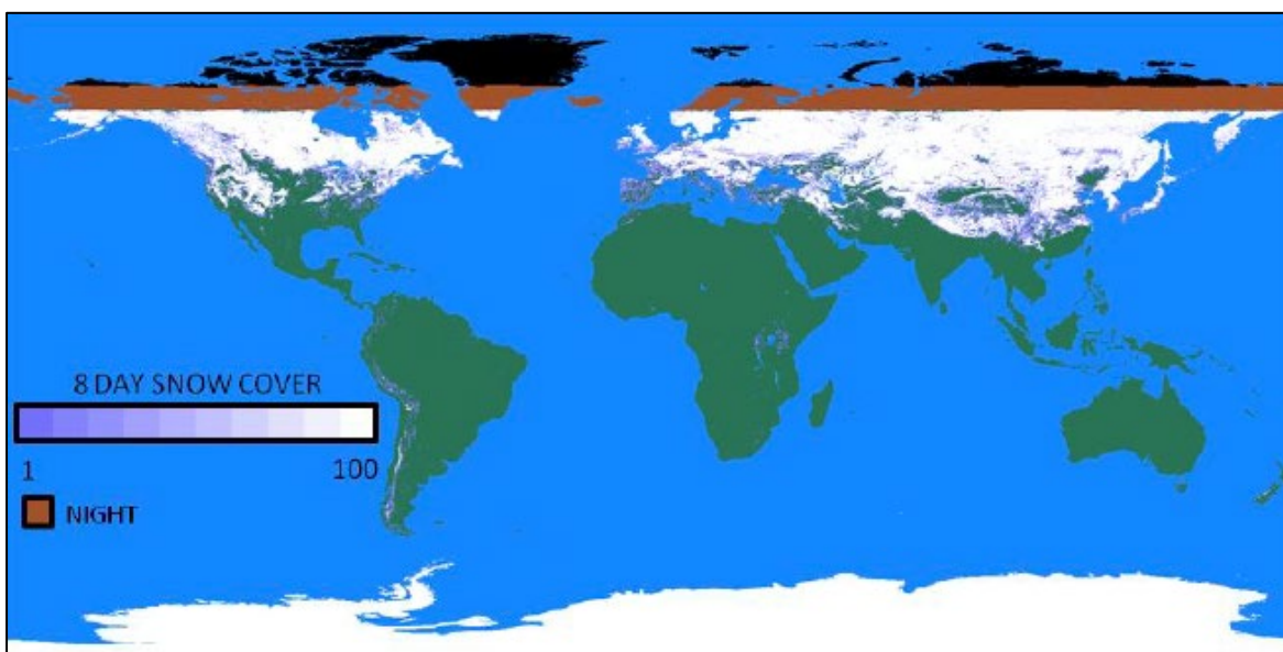
Figure 1. This MOD10C2 (MODIS/Terra) snow map shows the maximum percentage of eight-day snow cover mapped to a 0.05° CMG. The data was observed from 1 Jan thru 8 Jan 2003.
