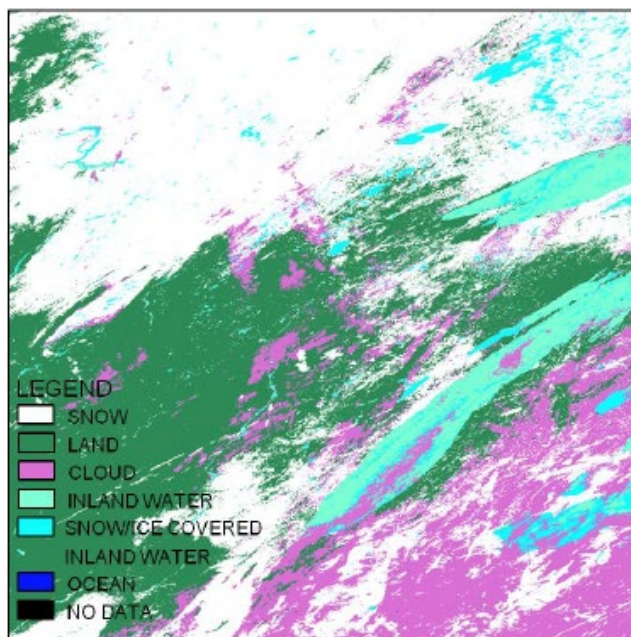
Figure 1. This figure shows MOD10A2 (from MODIS/Terra) eight-day snow cover extent for tile h11v04 observed 1 January 2003.
