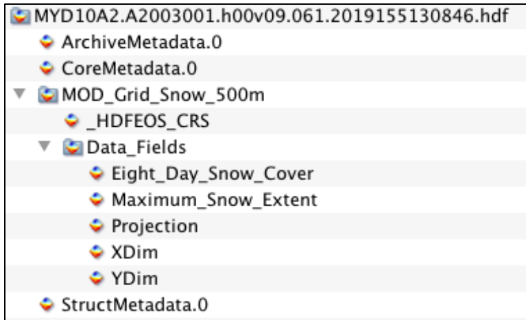
Figure 2. This figure shows the fields included in each data file as displayed with Panoply software.
