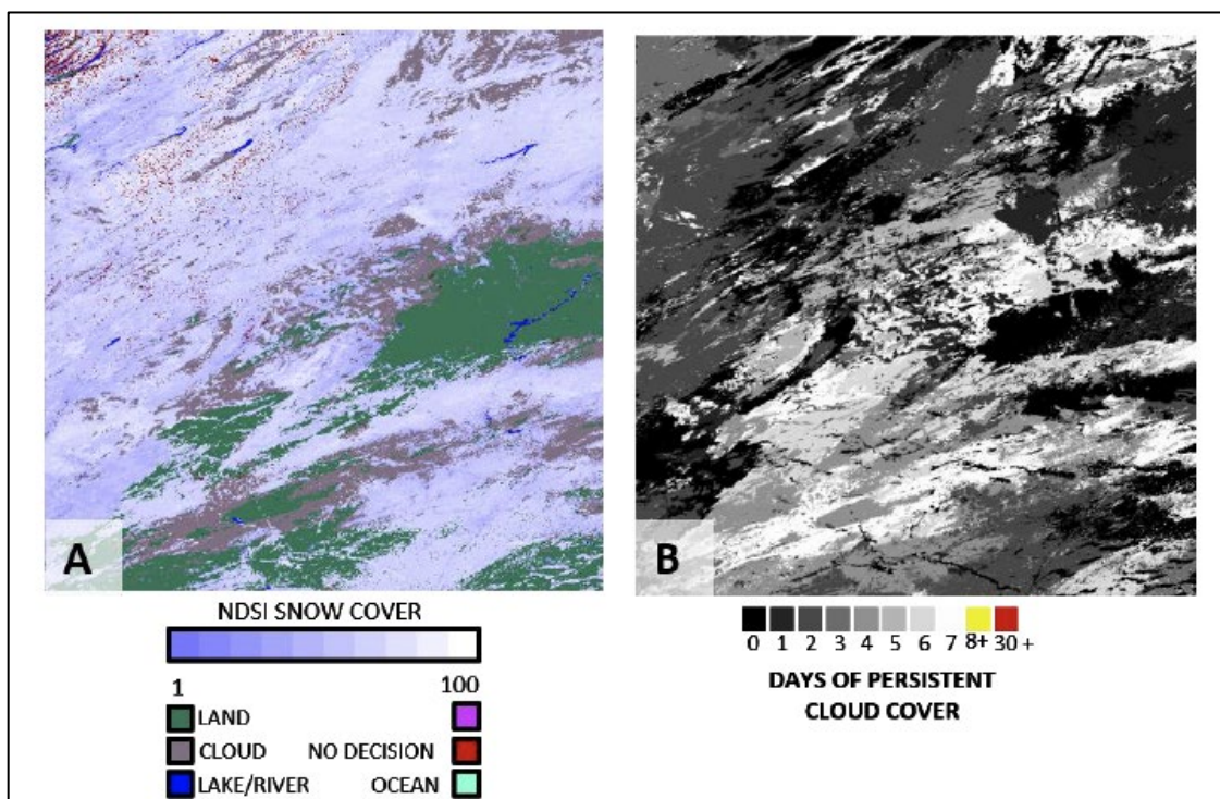
Figure 4. This figure shows CGF_NDSI_Snow_Cover (A) and cloud persistence (B) from MOD10A1F, tile h10v04, acquired 26 December 2017. The region shown extends from southern Nebraska to northern Montana. The unlabeled purple square in the legend represents 'Night'.
