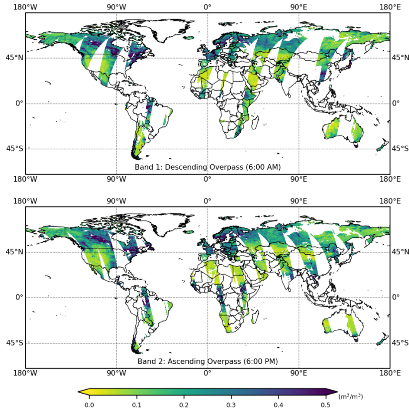
Figure 1. Example GeoTIFF
