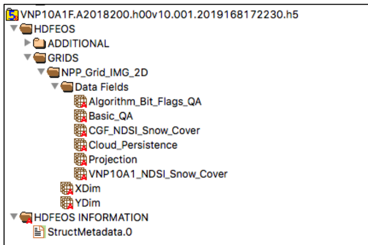
Figure 2. Parameters included in each V[NP|J1]10A1F file, as displayed with HDFView software. All data fields are two-dimensional except for Projection, which is an empty, attribute-only field.
