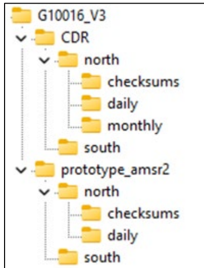
Figure 1. Directory Structure
