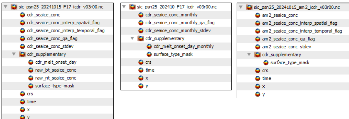
Figure 2. File Contents of a Northern Hemisphere CDR daily file (left), monthly file (middle), and AMSR2 prototype file (right).
