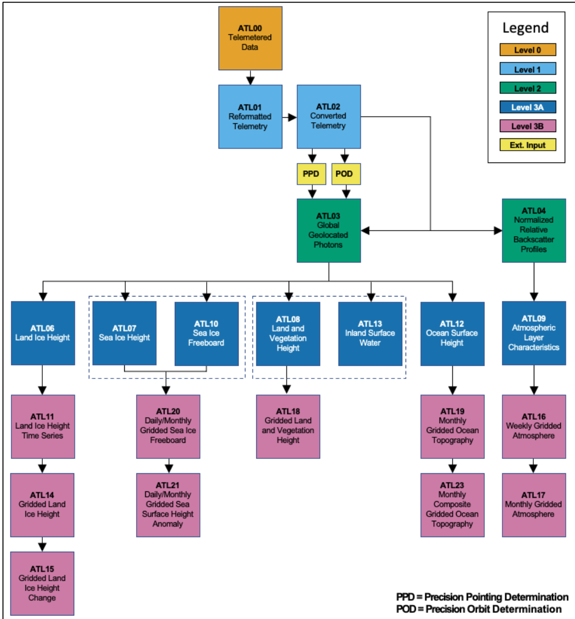
Figure 3. Schematic of the ICESat-2 data processing flow. The ATL01 algorithm reformats and unpacks the Level-0 data and converts it into engineering units. ATL02 processing converts ATL01 data to science units and applies instrument corrections. The Precision Pointing Determination (PPD) and Precision Orbit Determination (POD) solutions compute the pointing vector and position of the ICESat-2 observatory as a function of time.
