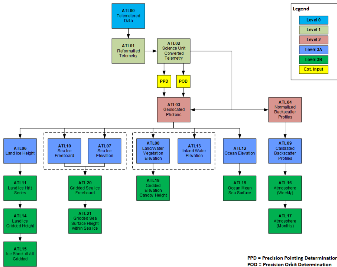
Figure 5. ICESat-2 data processing flow. The ATL01 algorithm reformats and unpacks the Level 0 data and converts it into engineering units. ATL02 processing converts the ATL01 data to science units and applies instrument corrections. The Precision Pointing Determination (PPD) and Precision Orbit Determination (POD) solutions compute the pointing vector and position of the ICESat-2 observatory as a function of time. ATL03 acts as the bridge between the lower level, instrumentation-specific products and the higher-level, surface-specific products.
