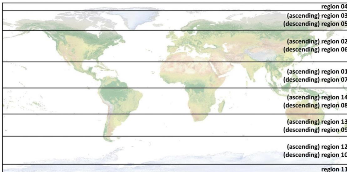
Figure 3. ATL06 region/granule boundaries.
