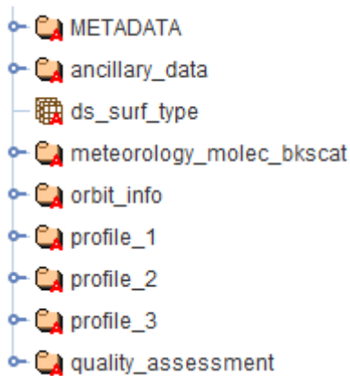
Figure 3. Top level data groups as shown in HDFView.
