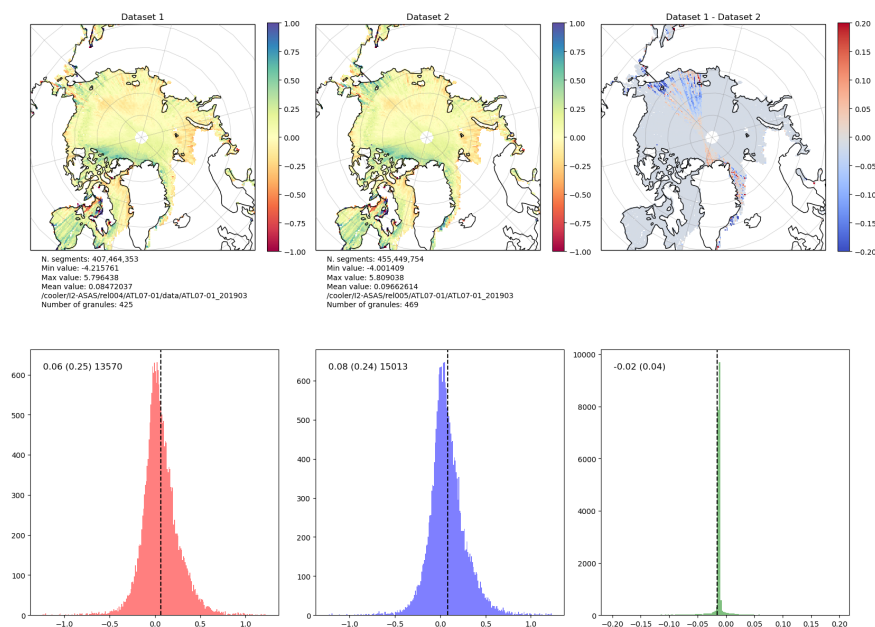
Figure 6: gridded maps (top) and histograms (bottom) of Arctic sea ice heights ( ssh\_flag = 0 ) from ATL07 during March 2019. Dataset 1: rel004, Dataset 2: test rel005. Note the difference in regions where the PODPPD flag = 4. Due to the change in along-track distance/spatial sampling during off-pointing scans it is challenging to determine any underlying bias in these data.
