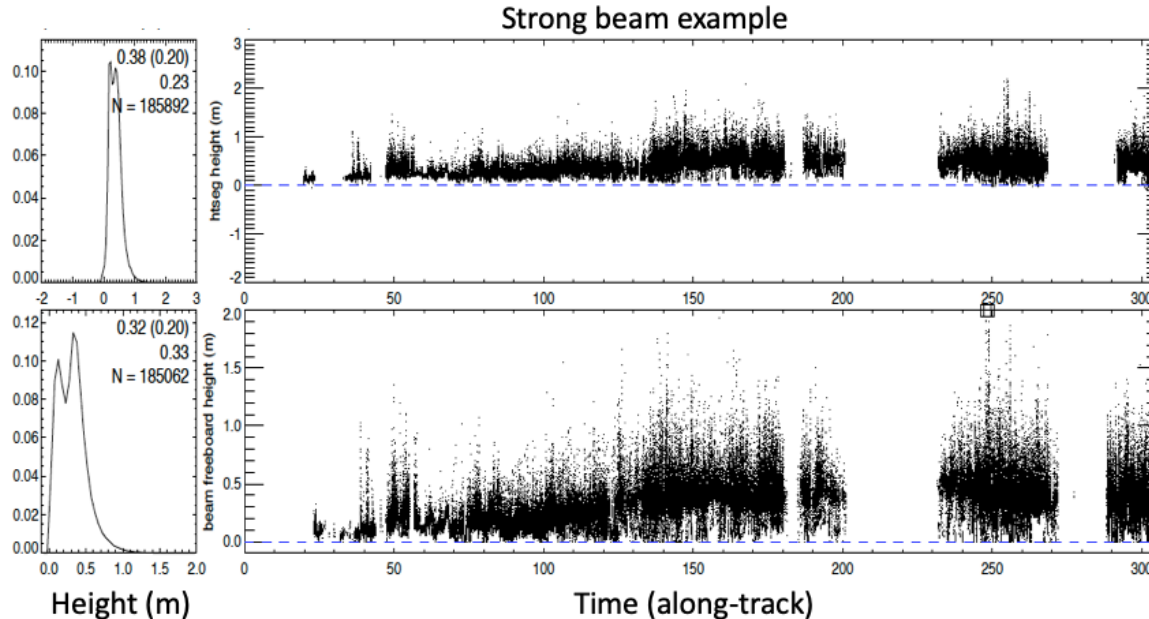
Figure 1: example ATL07 (top) and ATL10 (bottom) granule
