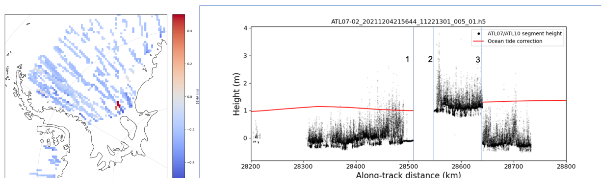
Figure 7: (left) gridded composite of ATL10 Sea Surface Height Anomalies (SSHA) from Dec 1-22, 2021, (right) ATL07 heights (black markers) for a granule extending over the Weddell Sea (over the positive SSHA shown on the left). ATL07 is missing between vertical lines 1 and 2 due to the presence of an iceberg and the effect of the coarse height filter (confirmed by ATL03) while the ocean tides (~1 m, red line) are missing between lines 1 and 3 resulting in the unphysical step-change in ATL07 between lines 2 and 3.
