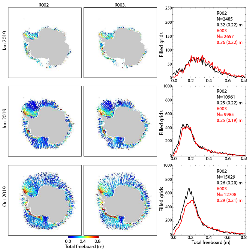
Figure 3: Same as previous figure except for the Antarctic.
