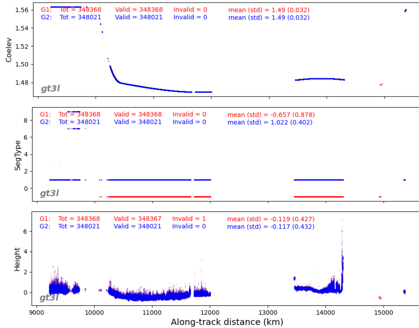
Figure 5: G1: rel005 test data, G2: rel004 data. Note the lower coelev angle after ~10000 km (in radians, top panel) indicates off-pointing in both datasets which in G1 (test rel005) triggers an invalid surface segment type (SegType = -1) with heights (bottom panel) unaffected.
