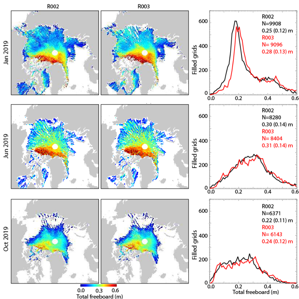
Figure 2: Changes in coverage and freeboard distributions of the Arctic Ocean sea ice cover in monthly composites of Jan, Jun, and Oct 2019. N is the number grid cells (25 by 25 km) that contains freeboard estimate. Numerical values are the mean (standard deviation) of the distributions. The distributions are not normalized and show actual population counts and provide an indication of the loss and gain of samples in each of the distribution bins.
