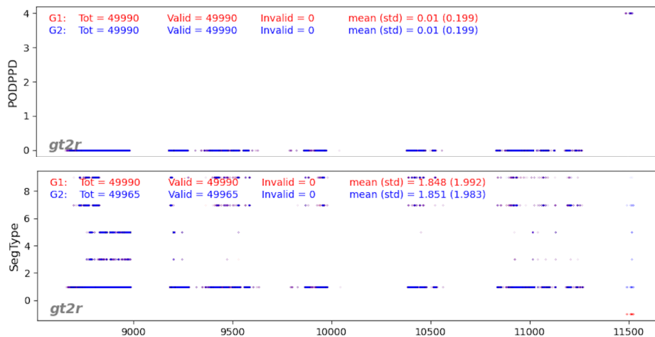
Figure 4: G1: rel005 test data, G2: rel004 data. Note the PODPPD flag of 4 in both datasets around 11500 km (top panel, right) which in the rel005/G1 test data triggers an invalid surface segment type (SegType = -1).
