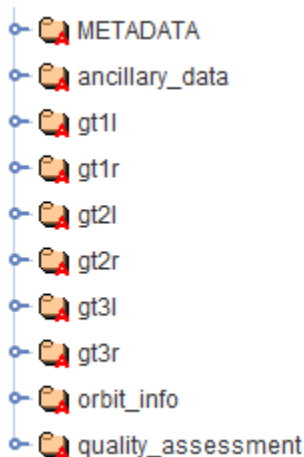
Figure 3. ATL13 data groups shown in HDFView.
