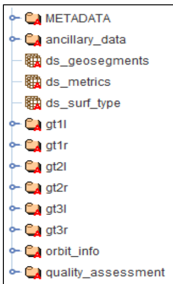
Figure 4. ATL08 data groups shown in HDFView.
