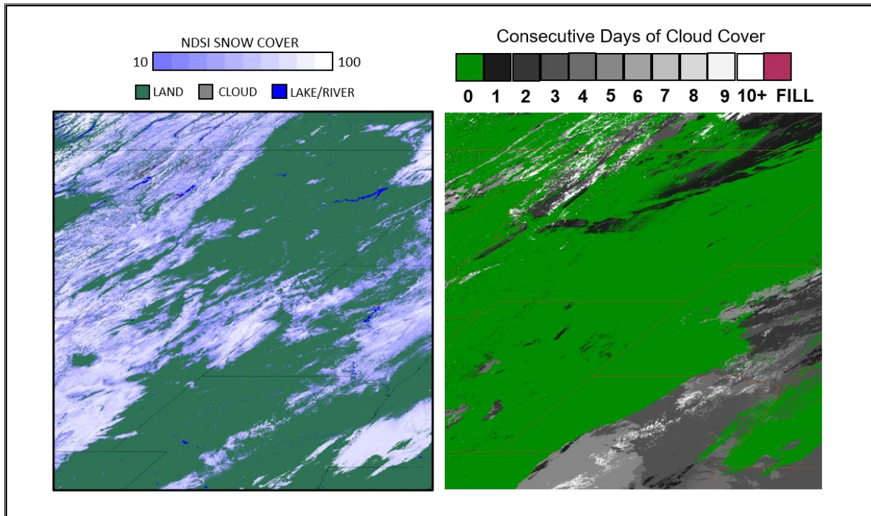
Figure 5. Cloud_Persistence from VNP10A1F.A2019013.h10v04.002.*.h5, 13 January 2019. The cloud persistence (right) shows regions clear skies (green) and where clouds have been observed on preceding days. Comparison with the CGF snow cover (left) (Fig. 4) reveals where snow cover observations are a few to many days old. The tile is projected in sinusoidal projection.
