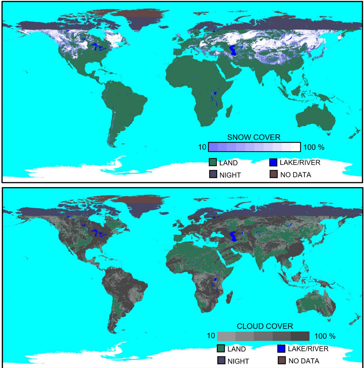
Figure 6. The VNP10C1 Snow_Cover map (top) and Cloud_Cover map(bottom) for 7 January 2019.
