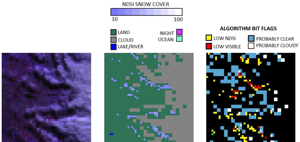
Figure 2. Example of snow commission error associated with cloud periphery and shadowed surfaces. Image is from the northern central region of VNP10 shown in Fig. 1. Left image is a false color display of VIIRS bands I2, I1, I3 (RGB) from the VNP02IMG swath corresponding to VNP10. NDSI_Snow_Cover from VNP10.A2019013.2048.002.*.nc (Fig. 1) is the center image. Selected data screens from the Algorithm_bit_flags_QA that prevent snow commission errors and the cloud mask confidence flags are shown in the right image.
