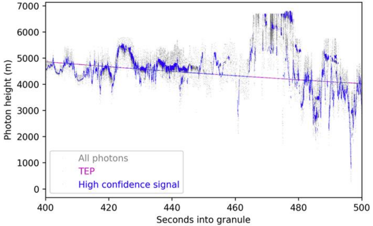
ATL03 Strong Beam Photons
