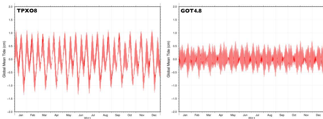
Figure 6-2. One year time series for 2011, of tide values averaged over the global oceans based on a time sequence of 1460, 1^{\circ} \times 1^{\circ} resolution global grids, computed every six hours. TPXO8 at left and GOT4.8 at right.
